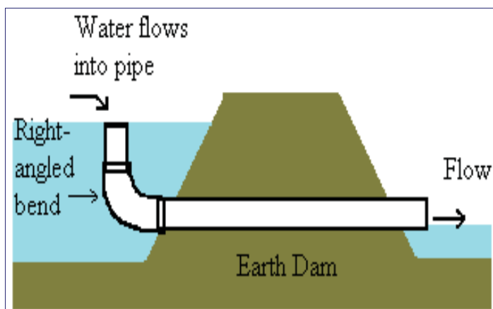
Fig 5: Basic pipe dam design
